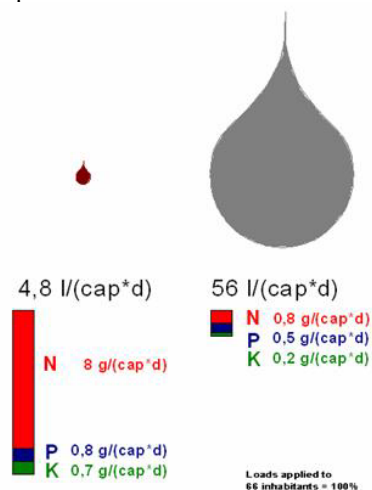
Figure 4.12. Volumes and content of nutrients of blackwater and greywater from a vacuum-biogas system in the residential area Flintenbreite, Germany.
