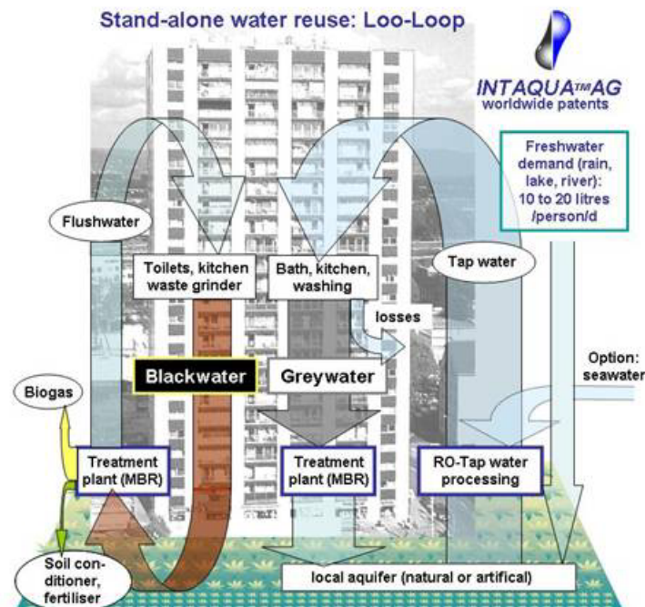
Figure 4.14. A system sketch of the blackwater loop.
