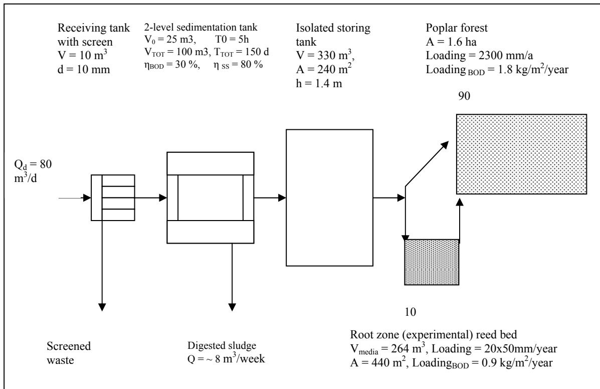
Figure 4.4. Principal sketch of the constructed system. Collected septic waste from households is transported to the receiving tank for screening. Pre- treatment takes place in a two-level sedimentation tank from which water is led to a sealed storage tank. From storage water is distributed by gravity to natural biological treatment units, the forest and the root zone wetland. Irrigation takes place year around and sludge is removed from sedimentation tank once a week.
